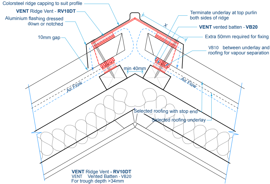
Fig B - RV10DT Application to Pitched Skillion Roof (any degree pitch)
