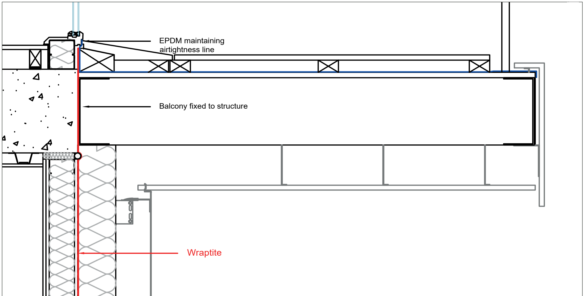
STEEL BALCONY, RAINSCREEN CLADDING
