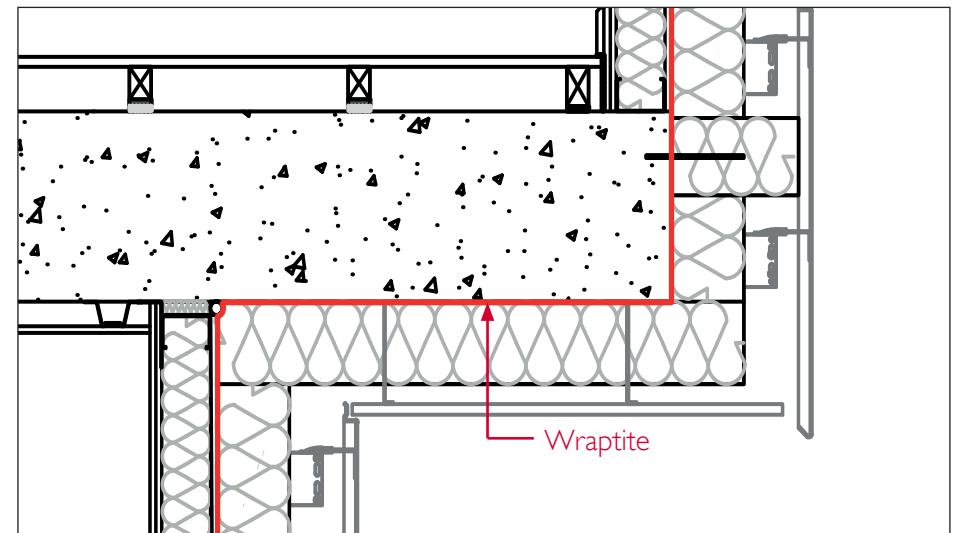
SOFFIT W. HORIZONTAL RAINSCREEN RAILS
