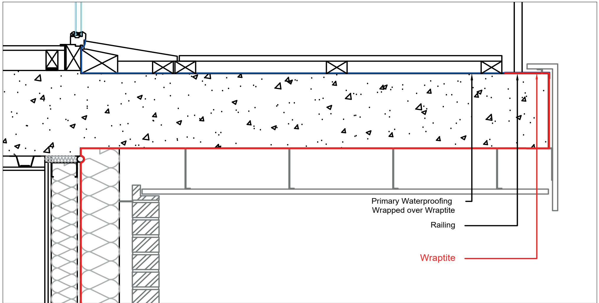
CONCRETE BALCONY, BRICK FAÇADE
