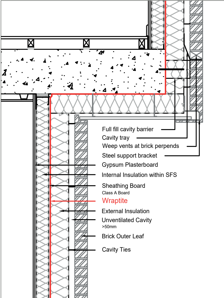
SOFFIT W. BRICK FAÇADE
