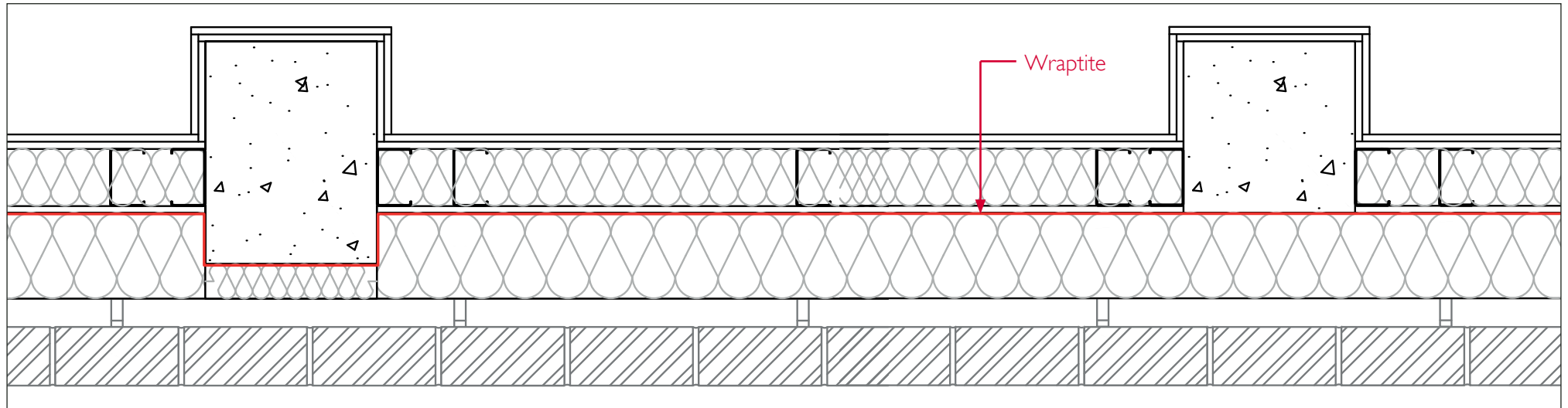
COLUMN - THROUGH SHEATHING BOARD BRICK FAÇADE
