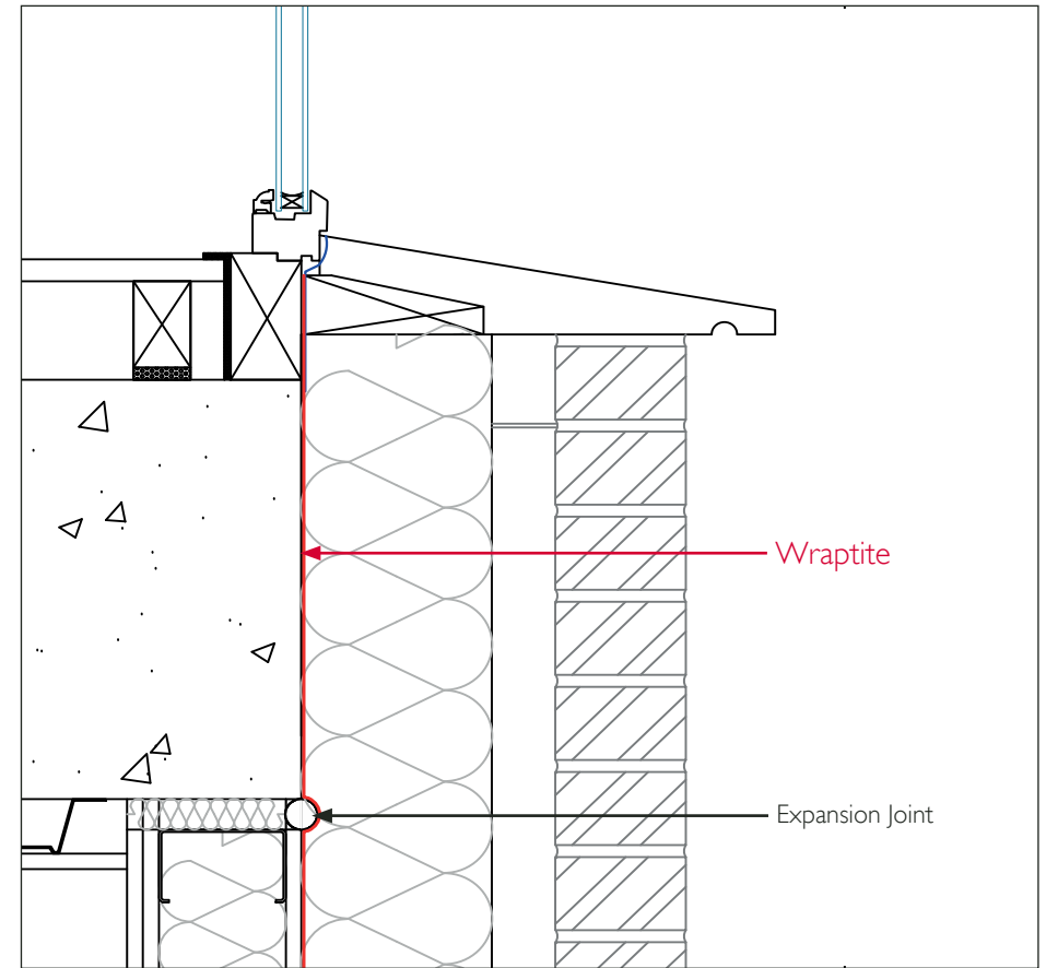
WINDOW SILL AT FLOOR LEVEL W. BRICK FAÇADE
