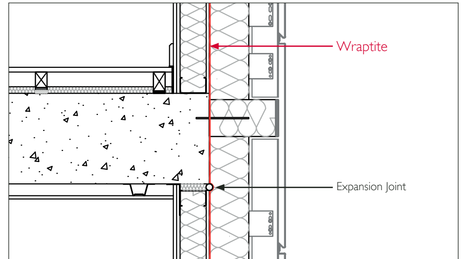
SLAB EDGE - VERTICAL RAINSCREEN RAILS
