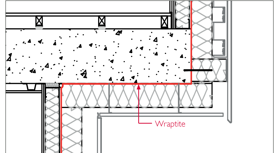
SOFFIT W. VERTICAL RAINSCREEN RAILS
