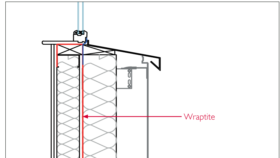
WINDOW SILL - HORIZONTAL RAINSCREEN RAILS
