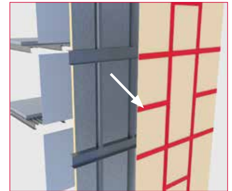
Fig.05: Wraptite Tape used to seal gaps between external sheathing boards.
