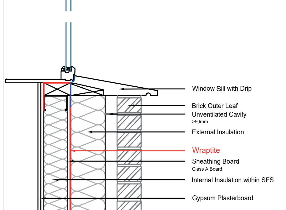
WINDOW HEAD & SILL - BRICK FAÇADE
