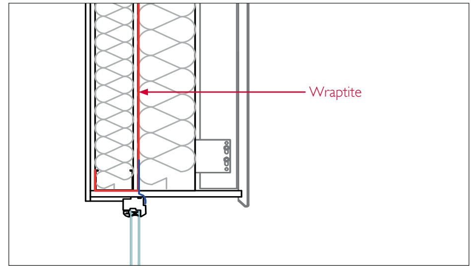
WINDOW HEAD - VERTICAL RAINSCREEN RAILS
