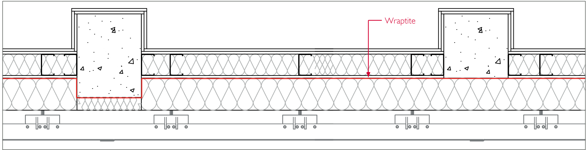
COLUMN - THROUGH SHEATHING BOARD RAINSCREEN CLADDING
