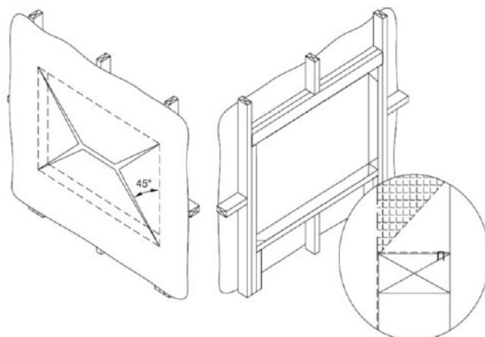
DETAIL 2
