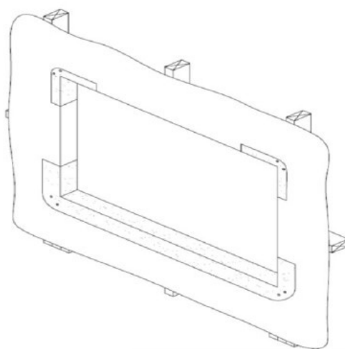
DETAIL 3
